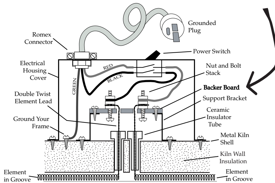
Top View of Connection Board Mounted on Kiln Wall
